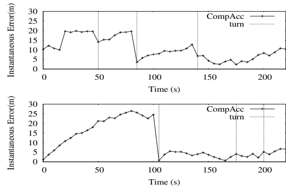
Fig. 12. CompAcc’s Instantaneous Error (IE) drops at path turns.
