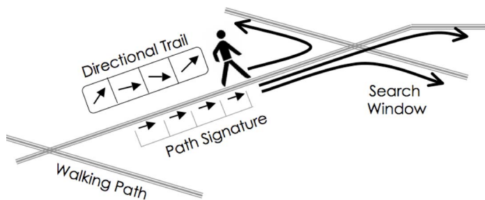
Fig. 4. CompAcc slides the path signature to a maximum of Search-Window steps, forward and backward. The sliding needs to turn into all possible directions within this window. For every step-wise slide, the “Dissimilarity” is computed between the given directional trail and the path signature. The path signature with minimum Dissimilarity yields the user’s current location.
