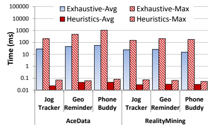
Figure 13: Time required to generate a plan on a Samsung Focus phone
