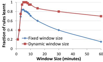
Figure 3: Effect of window size in batching
