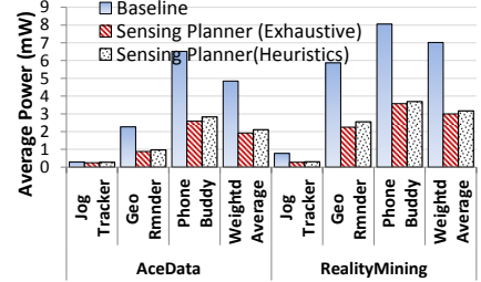
Figure 10: Energy savings by Sensing Planner
