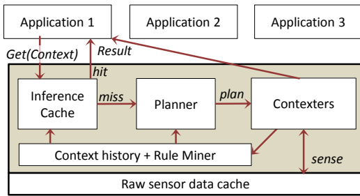
Figure 1: ACE Architecture
