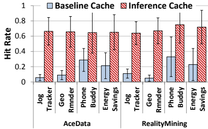
Figure 8: Hit rates and energy savings of Inference Cache
