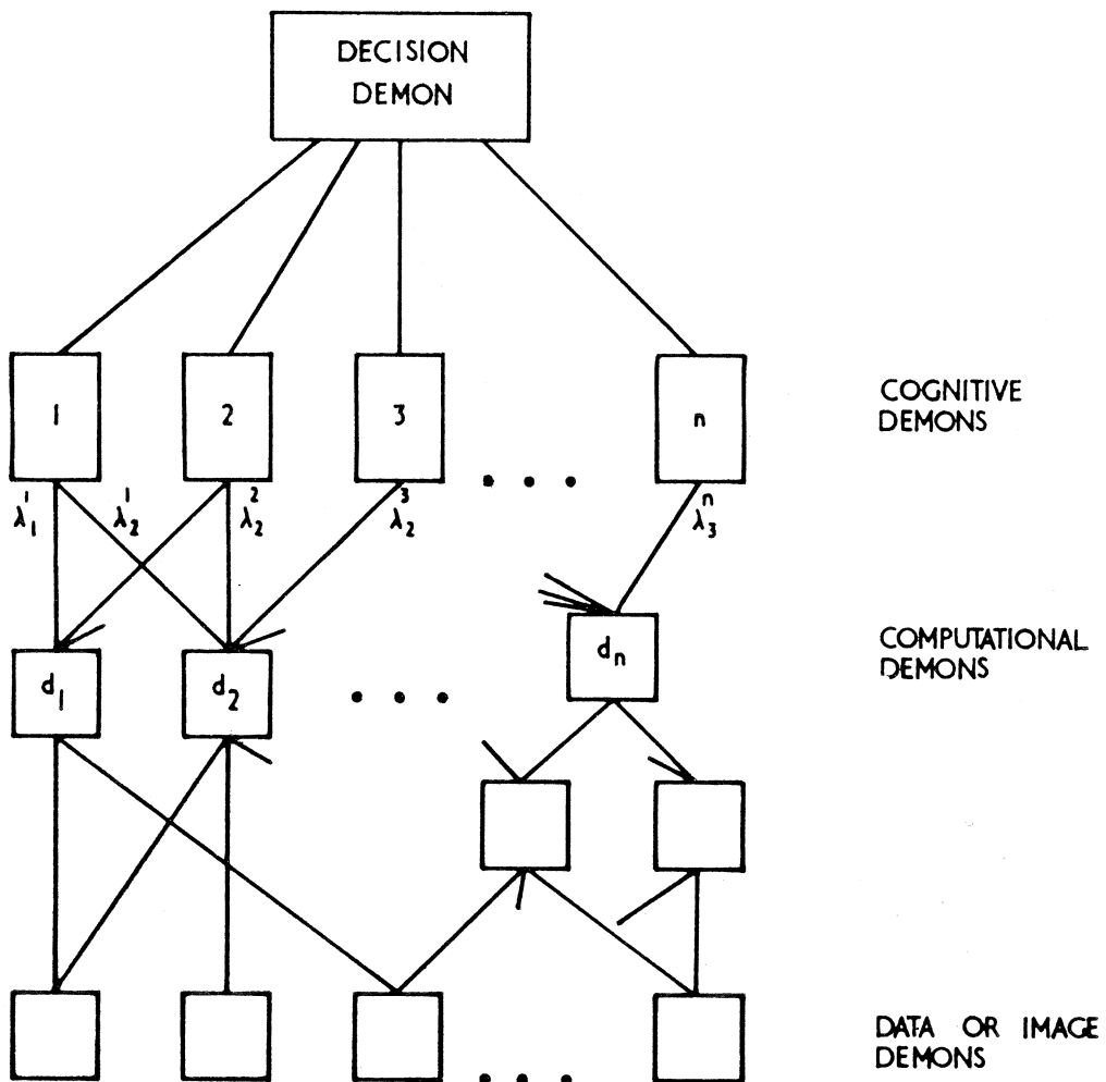
Fig. 3. Amended Pandemonium
