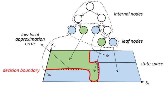
Figure 2: The decision tree can accurately approximate the original decision boundary.
