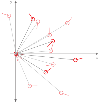
Figure 2. Two rotations of a 5-gon
