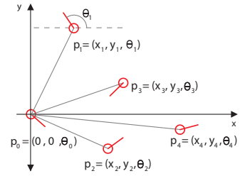
Figure 1. An n -gon where n = 5
