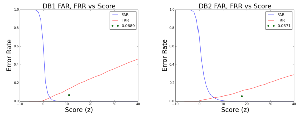
Figure 3. FAR vs FRR curves for our best performing matching scheme - n -gons all rotations. The ZeroFARs are .1266 and .1048 and the score thresholds are 10 and 17 respectively.
