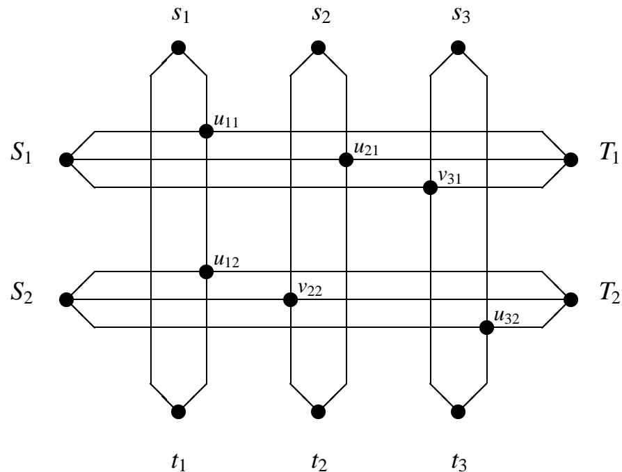
Figure 3: Construction in the proof of NP-completeness of DISJOINT CONNECTING PATHS for the formula (x_1 \vee x_2 \vee \bar{x}_3) \wedge (x_1 \vee \bar{x}_2 \vee x_3) .
