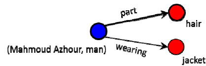
Figure 6. Merged Association Graph.
