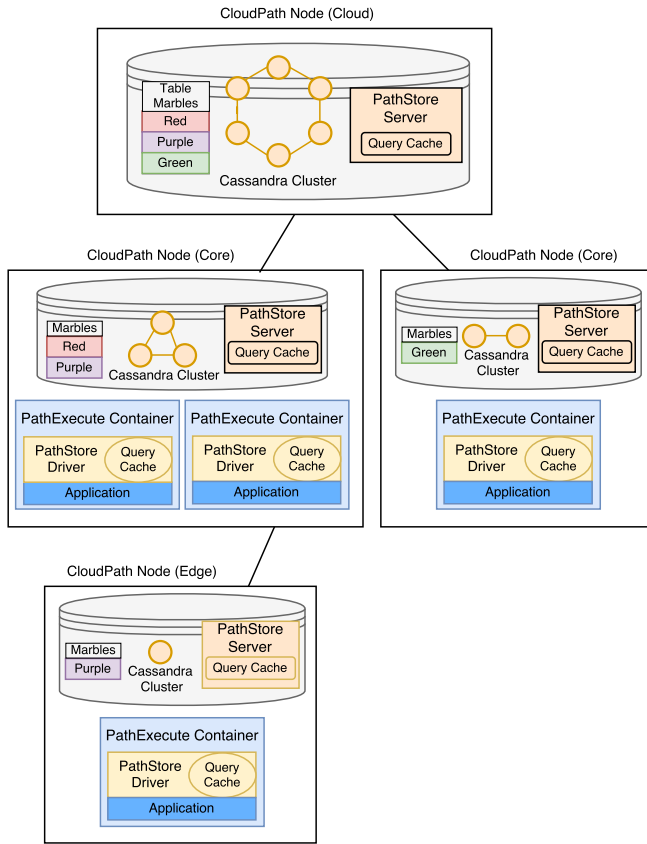
Figure 4: PathStore Architecture
