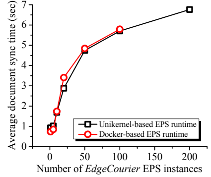
Figure 13: Unikernel-based vs. Docker-based EPS runtime: document sync time with EC EPS.
