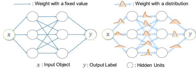
Figure 2. Illustration of Bayesian DNNs with a 2-layer model. All weights in Bayesian DNNs are represented as distributions using SG-MCMC (right figure); rather than having fixed values (left figure), as provided by classical stochastic optimization methods. The SG-MCMC learns correlated uncertainty jointly on all parameters, where (right) associated marginal distributions are depicted.
