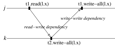
Figure 1. Conflicting transactions
