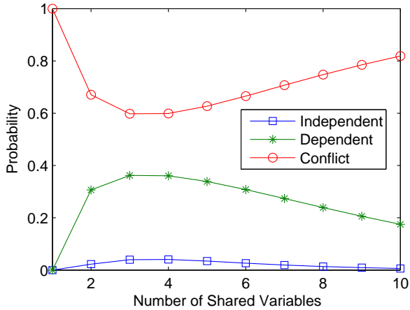
Figure 4. Probabilities of being independent/dependent/conflicting given the number of shared variables between two transactions
