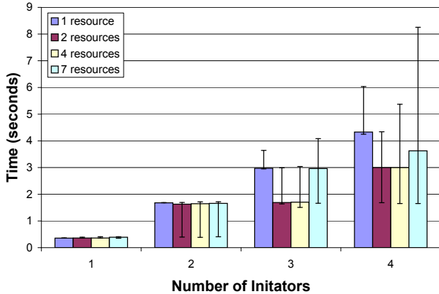
Figure 6. Settling time
