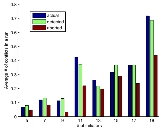
Figure 9. Conflict detection in TRANSACT
