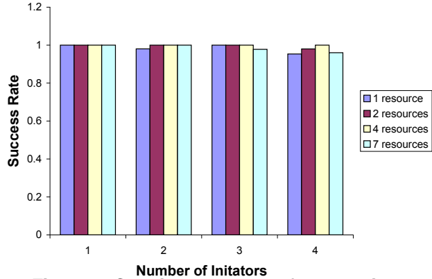
Figure 7. Consistency rates of transactions
