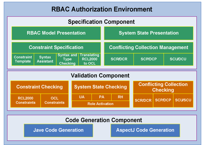
Figure 8: Structural overview of the RAE.
