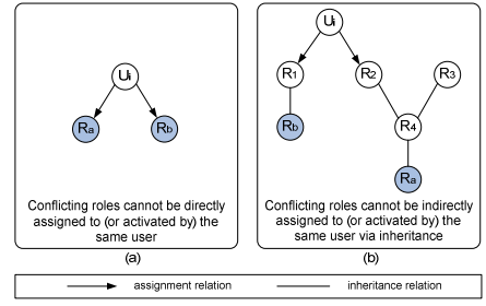
Figure 5: Conflict checking for SOD.
