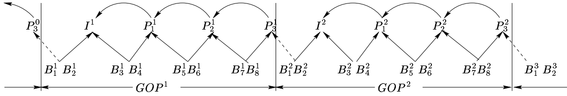
Figure 2: A Sample Pattern of MPEG Frame Dependency
