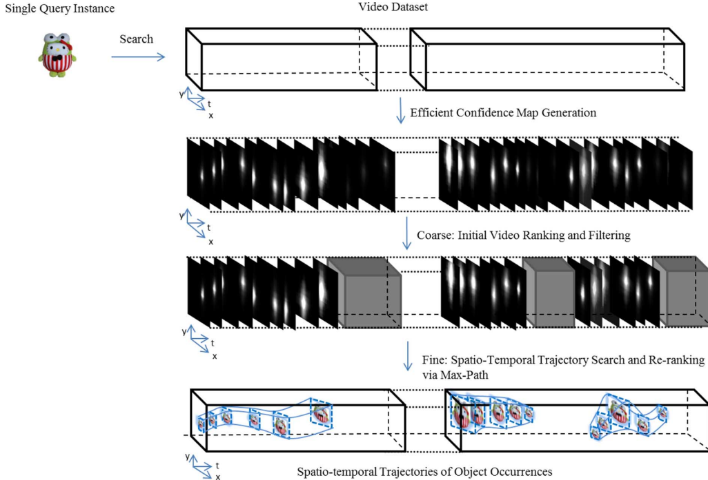
Fig. 2. Overview of proposed approach to find object trajectories in videos. Video keyframes are first matched with the query to produce confidence maps with pixel-wise matching score (2 nd row, Section III-C). Next, low confidence videos (the gray cuboids in the 3 rd row) are filtered by ranking videos based on the keyframe scores (Section III-D). Max-Path search then finds the globally optimal object trajectories in top ranked videos and re-ranks them according to the trajectory scores (Section III-B). Ground truth locations are highlighted in dashed blue boxes in the found trajectories (4 th row). Best viewed in color and magnification.
