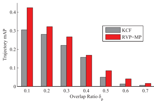
Fig. 6. Trajectory mAP: our RVP-MP method consistently outperforms KCF tracker [21] in a wide range of overlap ratio \delta_p .
