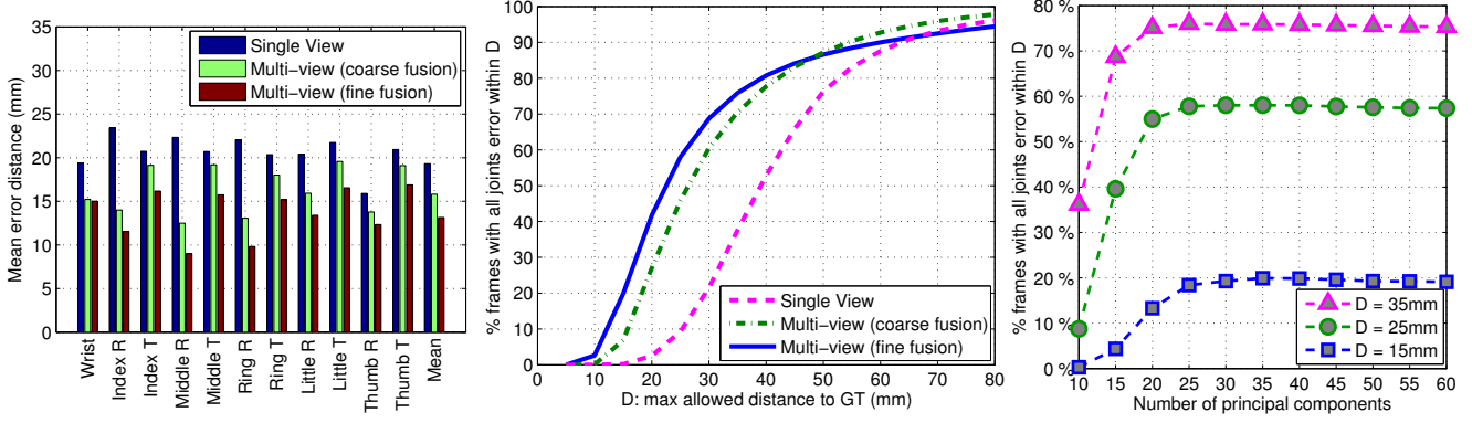
Figure 5: Self-comparison of different methods on the dataset in [19]. Left: the mean error distance for each joint across all the test samples (R:root, T:tip). Middle: the proportion of good test samples in the entire test samples over different error tolerances. Right: The impact of different number of principal components used in joint constraints on accuracy performance.
