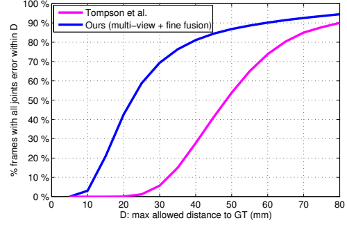
Figure 7: Comparison with the approach proposed in [27]. In this method, 14 hand joints are estimated. For fair comparison, in our method, 14 corresponding joints of 21 estimated joints are used to calculate the worst case accuracy.
