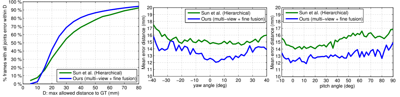
Figure 8: Comparison with the approach proposed in [19]. Left: the proportion of good test samples in the entire test samples over different error tolerances. Middle & right: the mean error distance over different yaw and pitch angles of the viewpoint. Our method holds smaller average errors in all of the yaw and pitch angles. The curves of the hierarchical regression method are cropped from the results reported in [19].
