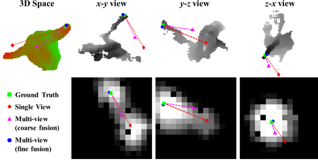
Figure 6: An experimental example for self-comparison. Top-left: 3D point cloud with ground truth and estimated 3D locations. Top-right: Projection images in three views. Bottom-right: Heat-maps of three views. The ground truth and estimated 3D locations are back-projected onto three views and their heat-maps for comparison. Lines indicate the offsets between ground truth and estimations.
