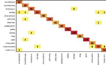
Figure 10: Confusion matrix of our method on PennAction dataset. Our method jointly learns 2D poses and heatmaps, and the complementary property between them alleviate the effect of noisy 2D poses. We further select one frame for each video and use CNN to extract deep features. Also, we encode annotated poses, which are provided by original dataset. Fused with these additional information, our method “(H1 + H3)*” outperforms all recent methods. The confusion matrix of our method is shown in Fig. 10, where most of ambiguities among actions are suppressed.
