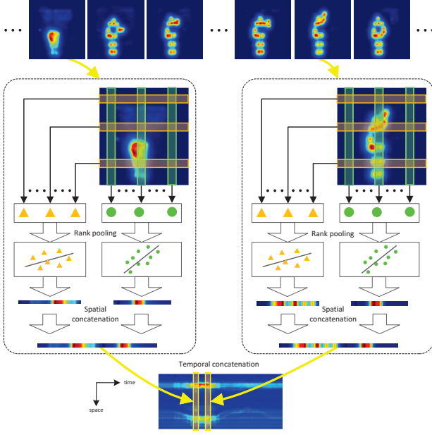
Figure 4: Generation of body shape evolution image via spatial rank pooling
