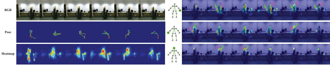
Figure 9: Visualization of 2D poses and heatmaps estimated from a video which denotes action “use a fan (with hand or paper)/feeling warm (49)”. We show the pose estimation maps of 8-th, 5-th, 1-st joint. On these pose estimation maps, green arrow points out the estimated position of joint, which is inaccurate. Meanwhile, pink arrow points to the region of heatmap which covers the ground truth of the joint position. We claim that heatmaps contain richer cues for inferring locations of joints when estimated 2D poses are inaccurate.
