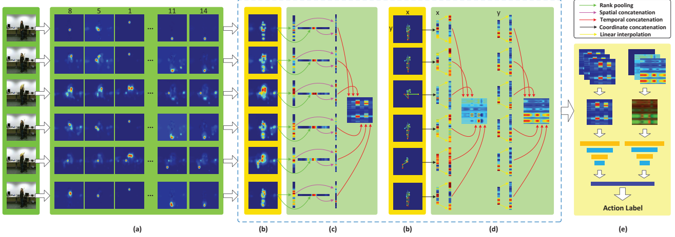
Figure 2: Overview of the proposed method. a) Convolutional pose machines predict pose estimation map of each body part. b) For each frame, pose estimation maps are aggregated to form a heatmap and a pose. c) Spatial rank pooling is proposed to describe the evolution of heatmaps as a body shape evolution image, which contains one channel. d) Body guided sampling is proposed to describe the evolution of poses as a body pose evolution image, which contains two channels. e) Deep features are extracted from both types of images and the late fusion result predicts final action label. Note that both images are converted to fix-sized color images to facilitate transfer learning.
