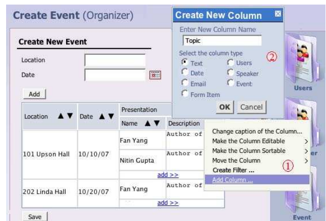
Figure 6: Adding the topic column to the presentation nested table. The resulting table is shown in Figure 2.
