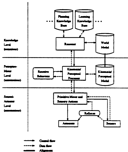
Figure 2: Schematic representation of the structure of a prototypical GLAIR-agent, an agent conforming to the GLAIR architecture.
