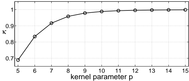
Figure 3: Contribution of the best matched local feature pairs, \kappa , Equation (7), in kernel K_{\mathcal{F}} with local jet features as a function of the kernel parameter p .
