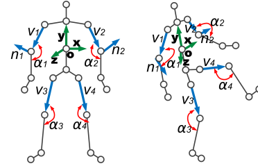
Figure 3. The representation of body part configurations.
