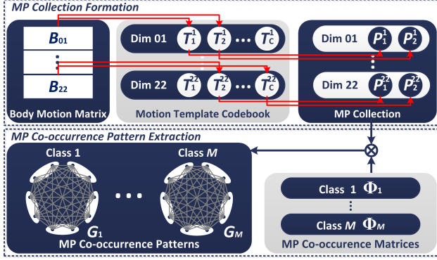
Figure 4. The upper row shows how an MP collection can be formed based on the extracted body motion matrix using the motion template codebook. The lower half is about the extraction of the MP co-occurrence patterns. Red arrows indicate the quantization procedure. The light grey blocks are reference repositories. In the block that shows the MP co-occurrence pattern, each action class should have 22 disjoint groups (each group is illustrated as an ellipse) with each corresponding to a dimension. However, we merely show five disjoint groups to make the diagram clearer. The notation used herein and the rest of the paper are defined in Table 1
