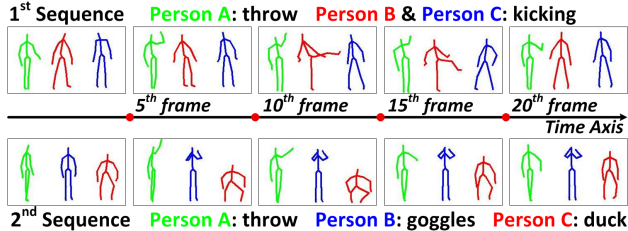
Figure 5. Sample frames from two test sequences of the Hybrid Actions3D dataset: The first row presents a hybrid-category test sequence involving two action instances, i.e. , Person A performing the single-person action "throw", while Person B and C are performing the two-person "kick" interaction. The second row presents a mono-category test sequence consisting of three single-person action instances, i.e. , Person A performing the "throw", B performing "goggles", and C performing "duck" action.
