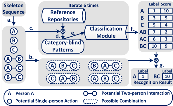
Figure 2. Main steps of CHARM. This example involves 3 persons ( i.e. , Person A, B, and C) and 6 potential actions. The recognition result indicates that A is performing a single-person action of Class 1, and B&C are performing a two-person interaction of Class 10.
