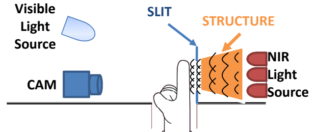
Figure 1. Layout of the fingerprint and finger vein capture device
