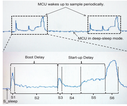
(b) Profiling of accelerometer sampling.
