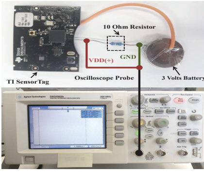
(a) Experimental setup for power measurement.
