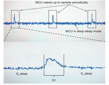
(c) Profiling of voltage sampling.
