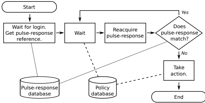
Fig. 2: Flowchart of the Continuous Authentication Process decision procedure.
