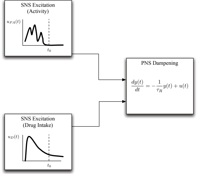
Fig. 3. ANS model of heart rate recovery.
