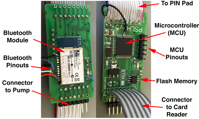
Fig. 2: The front and back of Skimmer S-03 with the major hardware components identified. We added the non-ribbon wires during analysis.
