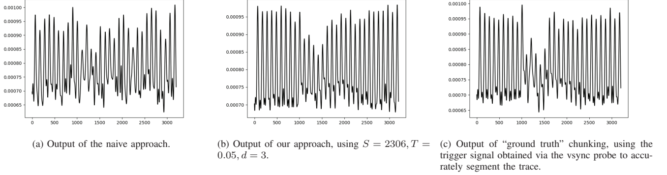
Fig. A.1: Comparing the outputs of the two chunking approaches on a Zebra of 30 periods, recorded using a parabolic mic (see Section III-A). The naive approach produces a signal whose amplitude is erratic and bears less resemblance to the one of the ground truth, even though it is using as input the exact refresh rate (up to 0.0001 s), and even though this rate is entirely stable across this particular recording (there are no abnormally sized cycles).
