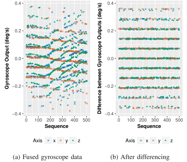
Fig. 4: Gyroscope data collected via JavaScript (iPad Air)
