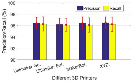
Fig. 11. Avg. precision/recall of four 3D printers.
