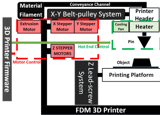
Fig. 2. The 3D printer hardware includes the stepper motors, the hot-end and the transmission systems [4].
