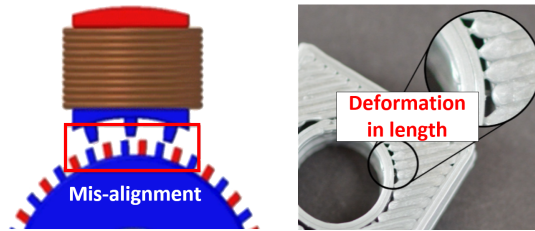
Fig. 5. One example of the geometric deformation in length caused by the random mis-alignment of the stepper motor.
