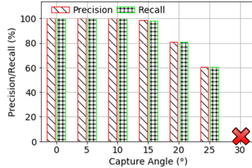
Fig. 16. The performances under different capture angles.
