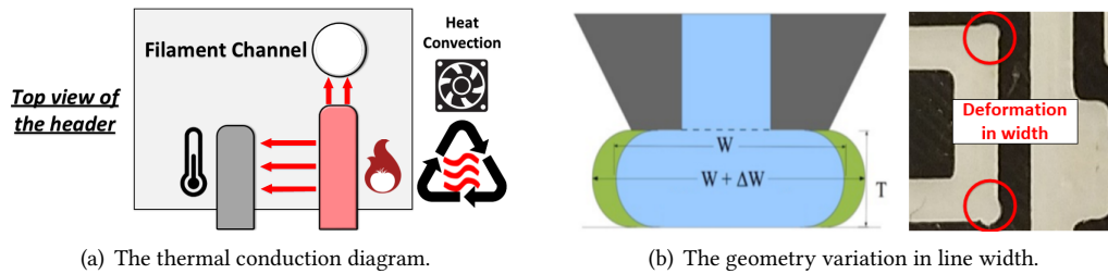
Fig. 6. The deviation in the temperature control system and the thus-derived small deformation.
