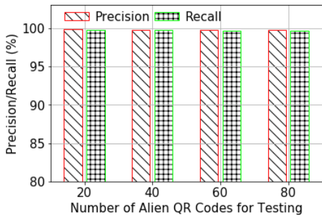
Fig. 13. Avg. precision/recall for alien QR codes.
