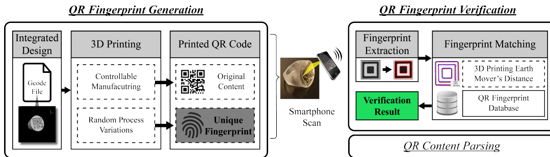
Fig. 4. The end-to-end cyber-physical solution of QR code fingerprint generation and verification. Note that the QR code contains two levels of information: the unique fingerprint and the original content.
