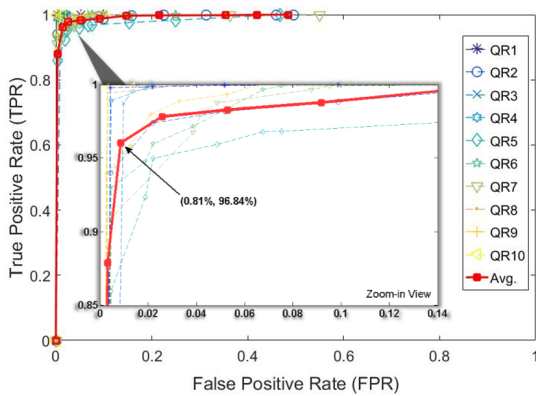
Fig. 9. The ROC curves of the QR codes.
