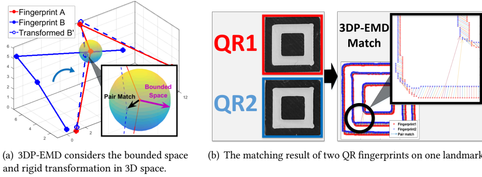
Fig. 7. The concept and demonstration of 3DP-EMD for QR fingerprint matching.
