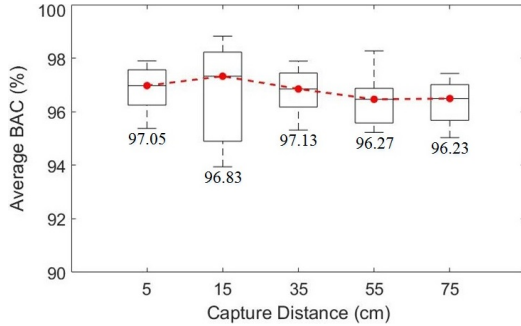
Fig. 15. Avg. BAC under different capture distances.
