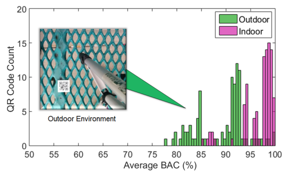
Fig. 18. Indoor and outdoor performance.
