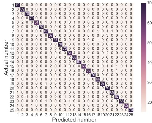
Fig. 10. The confusion matrix of 25 QR codes.
