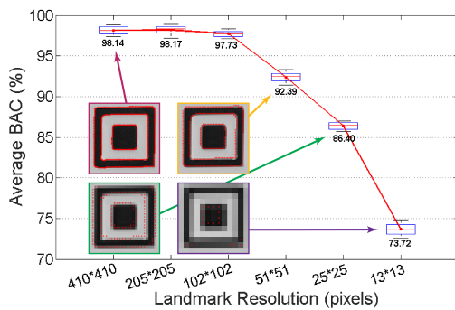
Fig. 17. Avg. BAC under different landmark resolutions.
